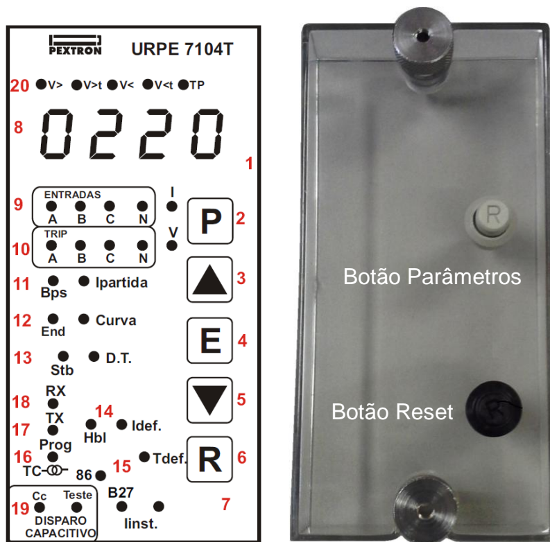
Figura 9: Painel frontal
